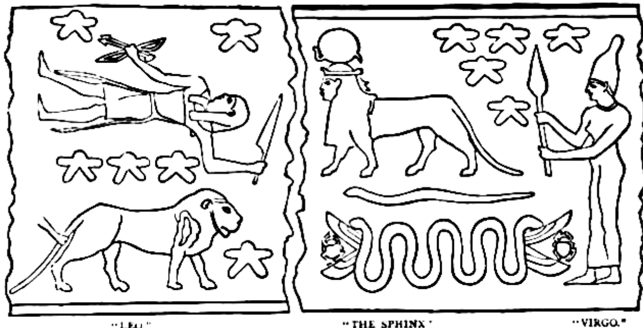
The Signs of LEU and VIRGO, from the ceiling of the Portico of the Temple of ESKEN, showing the SPHINX between, marking the beginning and end of the Zodiac
